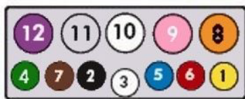
12 Pin Flat Socket
